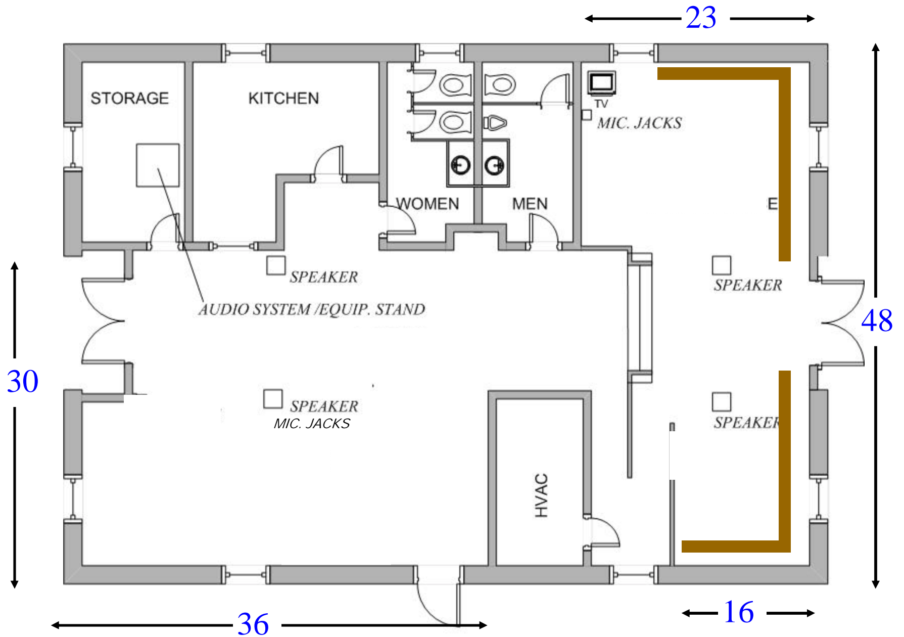
Rock Barn Floor Plan
